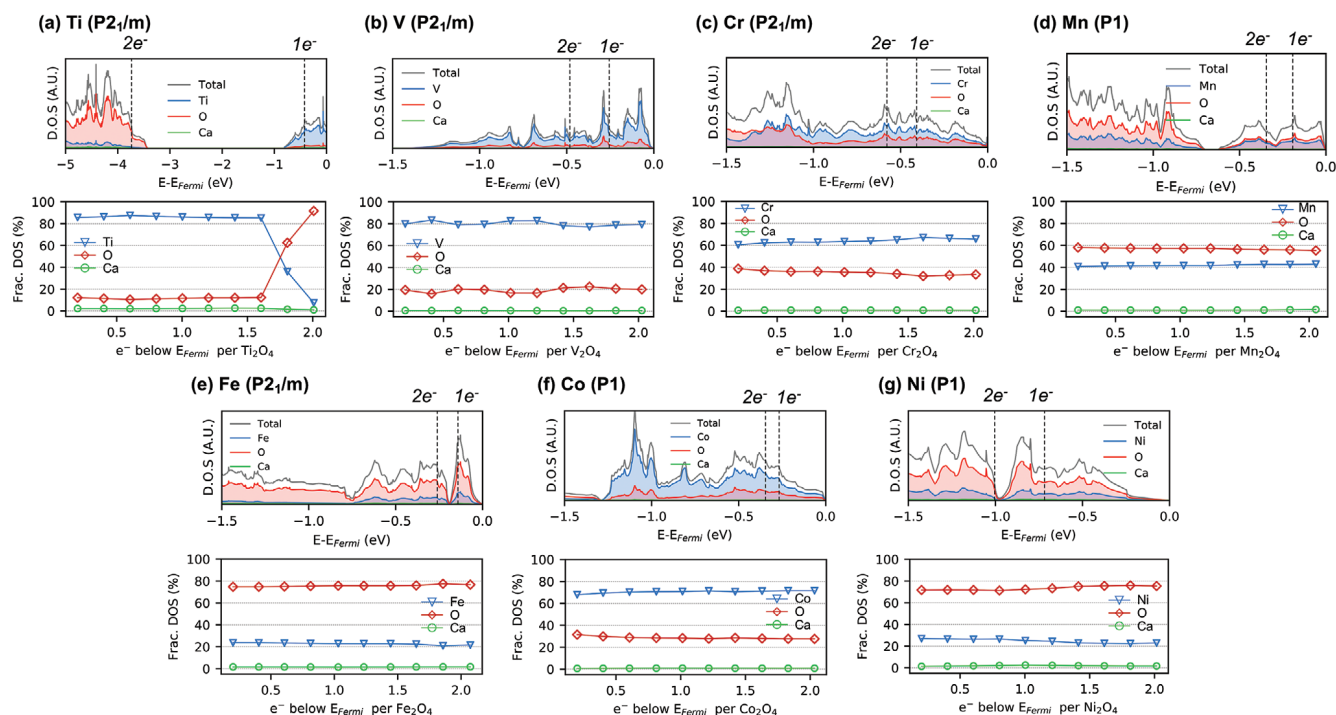
Figure 4. Atom-PDOS and the contribution of each species to total DOS of the various TM: a) Ti, b) V, c) Cr, d) Mn, e) Fe, f) Co, g) Ni substituted \text{CaTM}_2\text{O}_4 . In the PDOS plot, the grey, blue, red, and green represent the total DOS, TM PDOS, O PDOS, and Ca PDOS, respectively. The DOS is in an arbitrary unit (AU). The dashed lines indicate the energy levels where the total number of electrons from Fermi energy are one and two, respectively. The contribution of PDOS to the total DOS was sampled approximately every 0.2e^- and the fraction of each species in total DOS is plotted below the PDOS plot.
