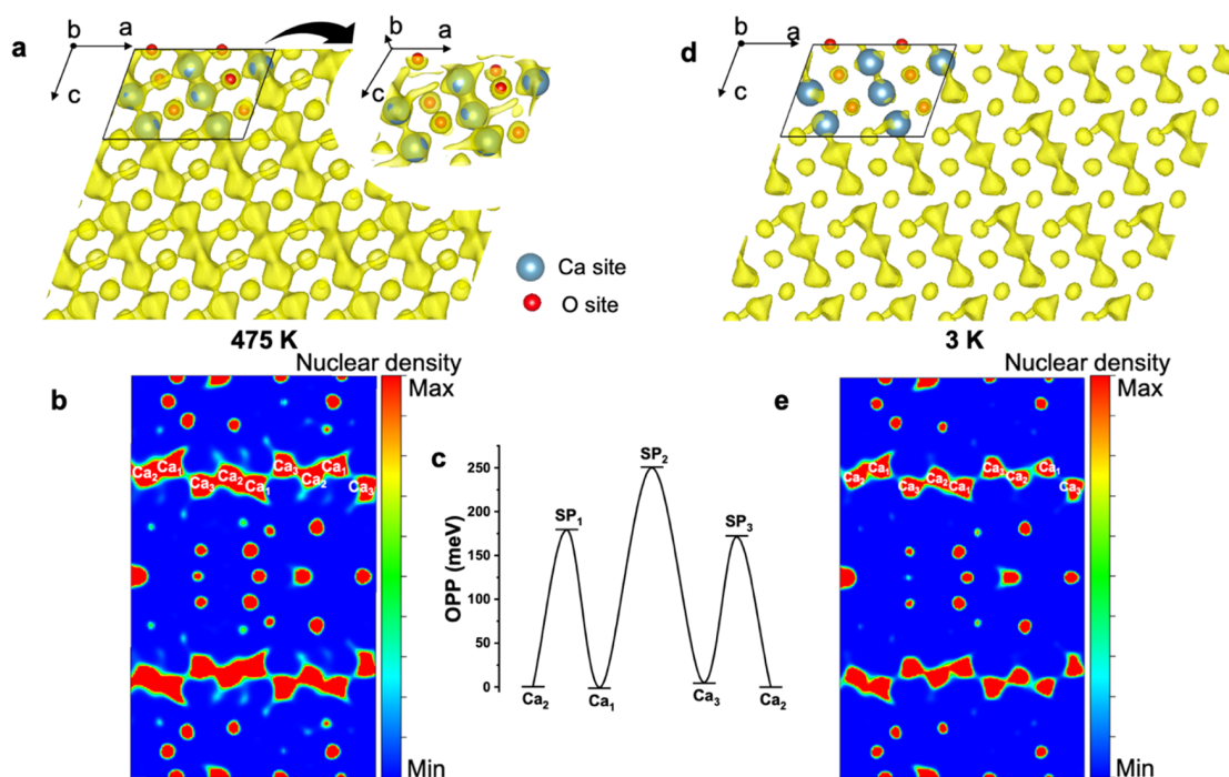
Figure 2. (a) Nuclear density isosurface plot obtained by an MEM analysis on the NPD data at 475 K shown in the Ca layer down the [010] direction (surface threshold, 0.03 fm/Å 3 ). In the unit cell, Ca and O sites are shown as blue and red balls, respectively. The inset presents a slightly tilted isosurface view of the Ca layer. (b) Nuclear density map at 475 K sliced in the (232.11, 1, −110.309) plane with a distance from the origin of 2.47616 Å. (c) Effective one-particle potential profile along the 1D diffusion path, which is calculated from the nuclear density map at 475 K by assuming the validity of Boltzmann statistics. (d) Nuclear density isosurface plot at 3 K in the Ca layer down the [010] direction (surface threshold, 0.03 fm/Å 3 ). (e) Nuclear density map at 3 K sliced in the (232.11, 1 −110.309) plane with a distance from the origin of 2.47616 Å. The scale is the same as in panel (b).
